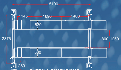
OVERALL DIMENSIONS
