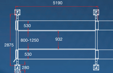
OVERALL DIMENSIONS
