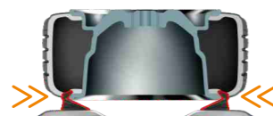
Outside clamping 12~26"
